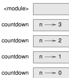
Figure 5.1: Stack diagram.
